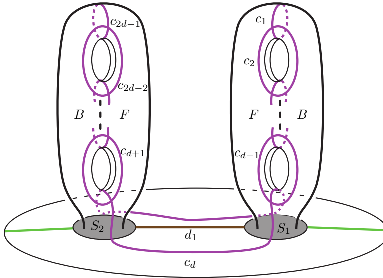
FIGURE 22. The surface \Sigma_{(2,1)} . The spin map r_2 can be seen by rotating the picture 180^\circ and then sliding the boundary clockwise back to where it began.
