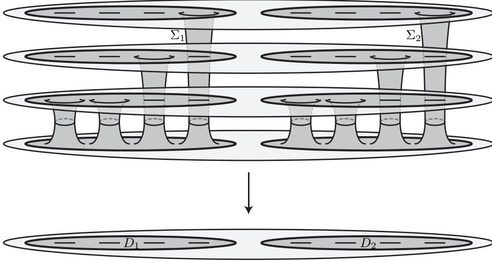
FIGURE 12. A page of the (2, 1) -cable of (\Sigma, id) when \Sigma has genus 1 and 4 boundary components. The two nodules \Sigma_1 and \Sigma_2 are shown in grey. The white regions are the 4 base components C_1, \dots, C_4 .
