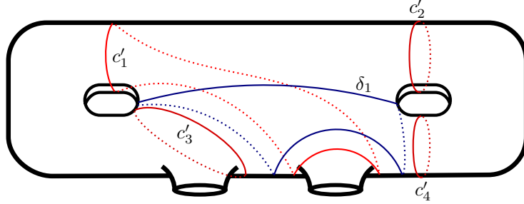
FIGURE 29. The Dehn twists involved in the lantern with \beta^{-1} and \partial_{\Sigma}^{-1} .
