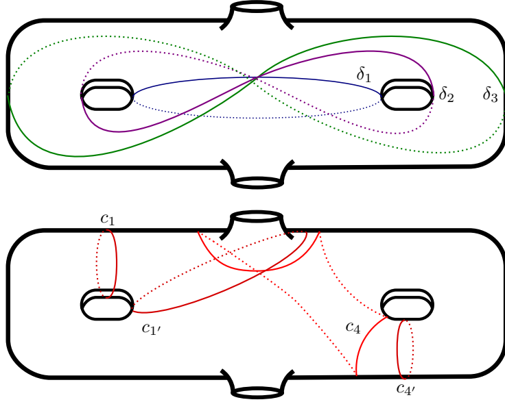
FIGURE 31. The Dehn twists in the factorization of the (2,2) -cable after sliding the boundary component on the right up the back of the surface to the top. The top diagram shows the curves \delta_1 , \delta_2 and \delta_3 , which give the final monodromy.
