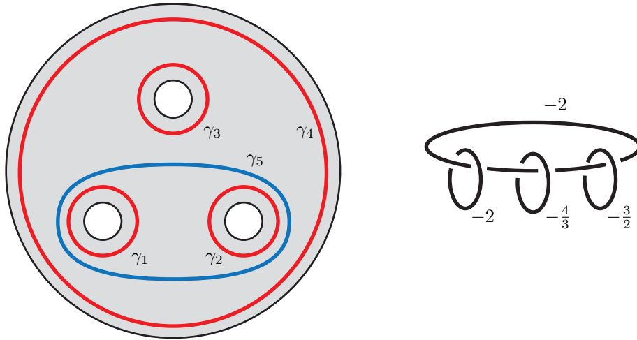
FIGURE 16. Left, planar surface with four boundary components and curves used to describe the monodromy in Example 6.9. Right the manifold constructed in the example.
