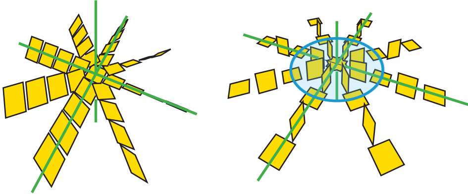
FIGURE 2. The contact structure \xi_{std} and \xi_{ot} with the overtwisted disk indicated on the right. (Figure courtesy of S. Schönenberger.)
