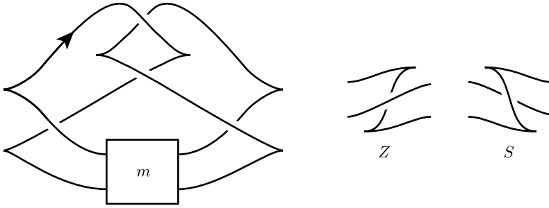
FIGURE 15. A Legendrian twist knot. The box is replaced with a tangle formed by concatenating m of the Z and S tangles shown on the right, in any order.
