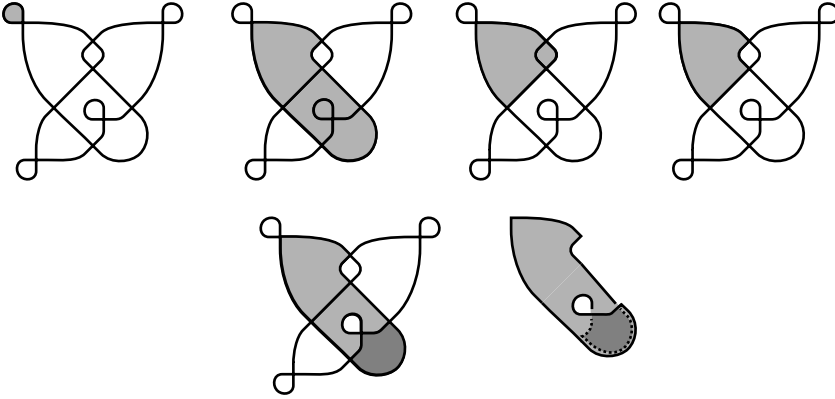
FIGURE 8. The five disks that go into the computation of \partial_{\Lambda_1} a_1 for the Chekanov example knot \Lambda_2 from Figure 7. The disk on the left of the bottom row is immersed, and the darker shaded part indicates where the immersion is two-to-one. The final picture on the bottom row is another view of this immersed disk: the boundary of the disk is slightly offset where the immersion is two-to-one to better indicate the overlapping region.
