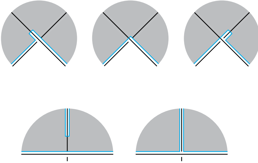
FIGURE 9. The new types of disks in \widehat{\Delta}(a; b_1, \dots, b_n) . Along the top row we see a disk with a branch point on the right and left, and in the center we see a non-convex corner; the result is that a disk with such a non-convex corner is in the interior of a moduli space of dimension larger than 0. On the bottom row we see a disk with a branch point moving toward the boundary of the disk, at which point it limits to the union of two disks.
