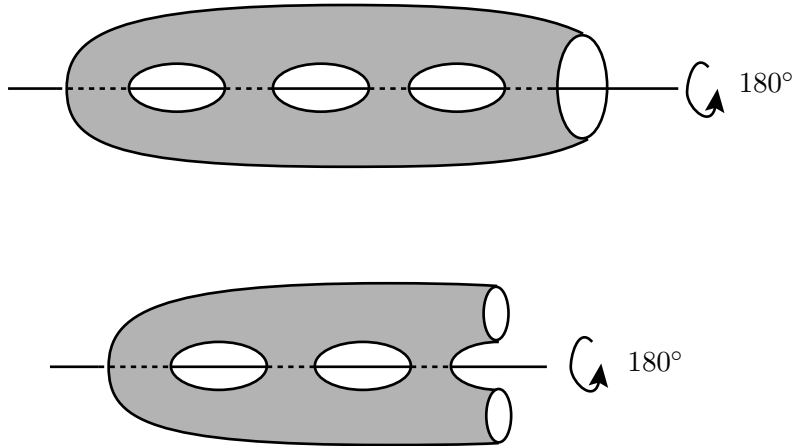
FIGURE 11. The hyper-elliptic involution h_1 top, and h_2 bottom.
