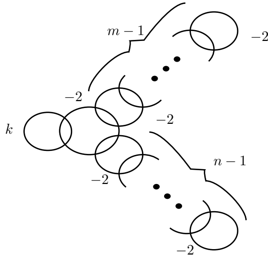
FIGURE 6. Handle decomposition of a 4-manifold X with \partial X = M_{m,n,k} .
