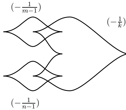
FIGURE 7. A contact surgery picture of M_{m,n,k} .
