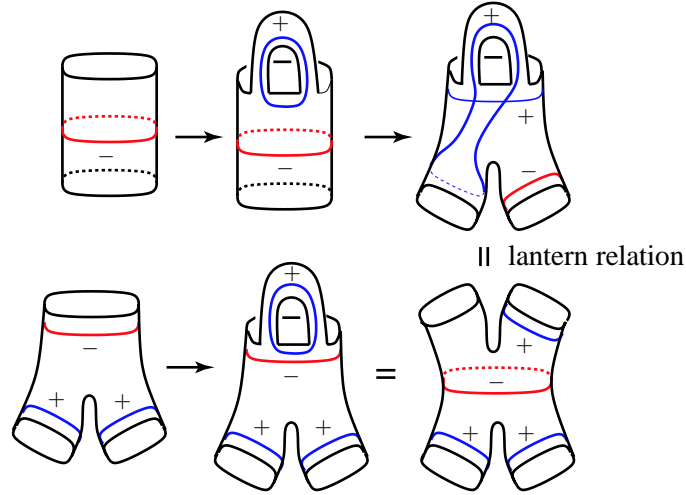
FIGURE 3. Positive stabilization of \text{ob}_1 twice (the top row) and \text{ob}_2 once (the bottom row).
